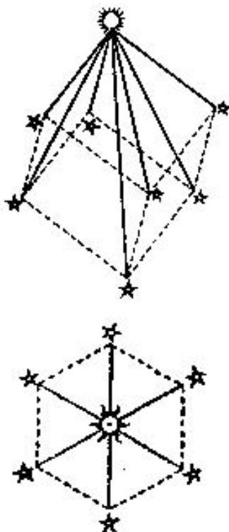
The cube in its isometric projection.
