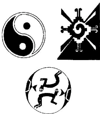
The Chinese Ying-Yang, Mayan Hunab Ku and Navajo symbol.
