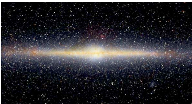
The Milky Way (photo © NASA)
