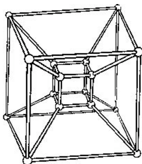
The Tesseract.
