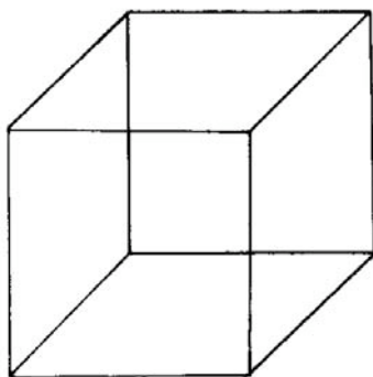
The Necker Cube
