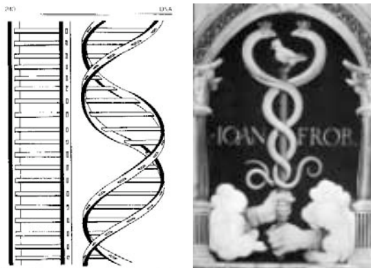
DNA molecule (left) and the caduceus.
