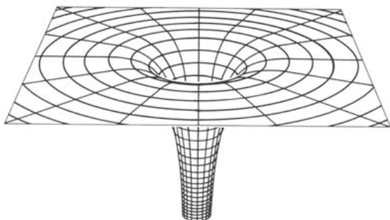
Theoretical illustration of a black hole.
