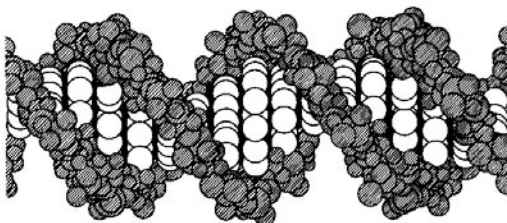
DNA molecule
